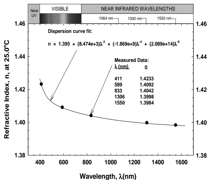
Refractive Index vs. Wavelength (25°C) NuSil Silicone Elastomer R-2615, Lot# 31426
